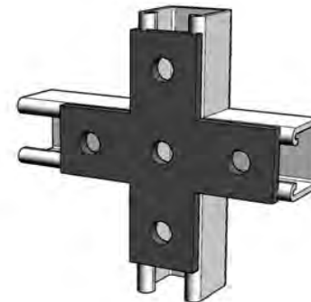
FIVE HOLE CROSS PLATE Stock No. 121P-HG
