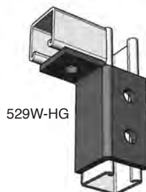
THREE HOLE 90° FITTING Stock No. 528W-HG 529W-HG Style Right Hand Left Hand
