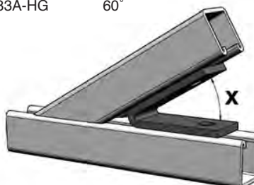
TWO HOLE CLOSED ANGLES Stock No. X Angle 279A-HG 30° 278A-HG 45° 276A-HG 60°
