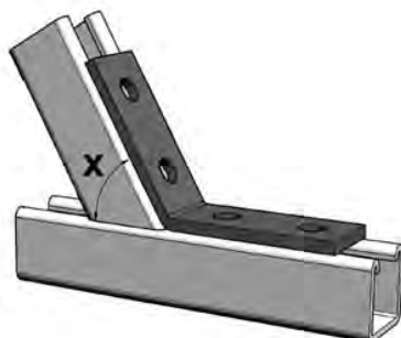
FOUR HOLE OPEN ANGLES Stock No. X Angle 265A-HG 30° 267A-HG 45° 269A-HG 60°
